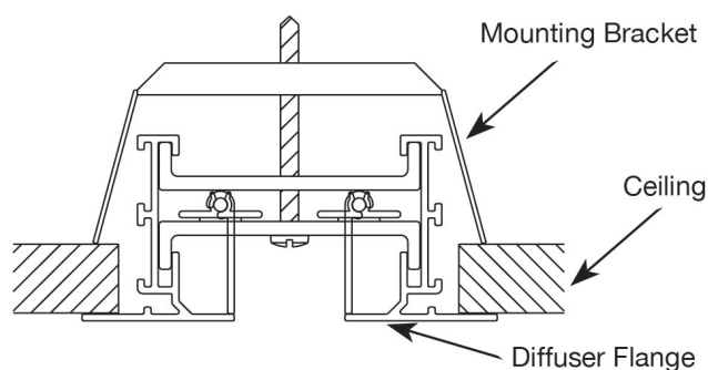
Figure 7. Diffuser Installation without Plenum
