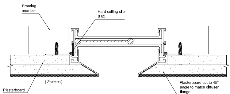
Figure 2: Plasterboard Installation (Border 55 ONLY)
