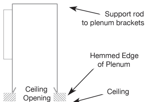
Figure 4. Concealed Fastening Plenum Installation
