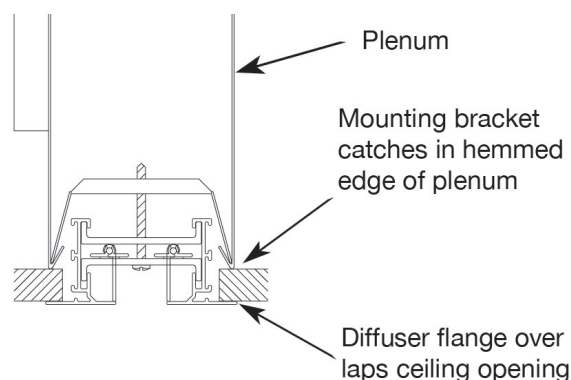
Figure 6. Diffuser Installation with Plenum
