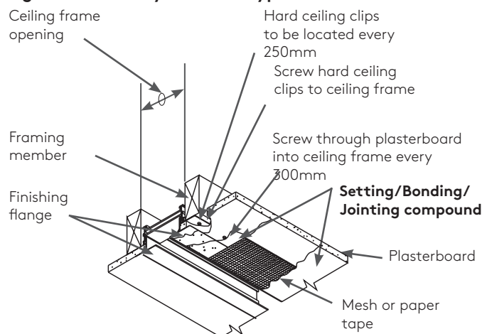
Figure 3: Summary of Border Type 22 Installation
