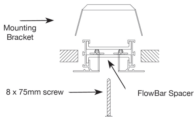
Figure 5. Bracket/Diffuser Assembly
