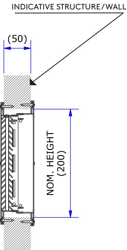
SECTION B-B
