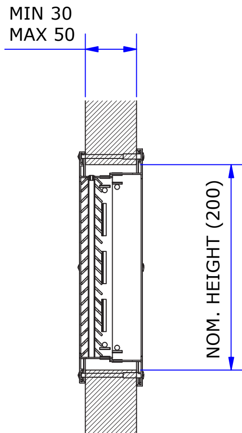
SECTION C-C
