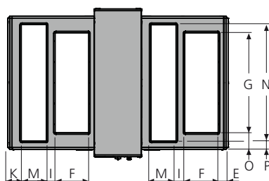
View from above. Shows the air handling unit's duct connections for supply air fan right down and left up
