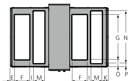
View from above. Shows the air handling unit's duct connections for supply air fan right up and left down
