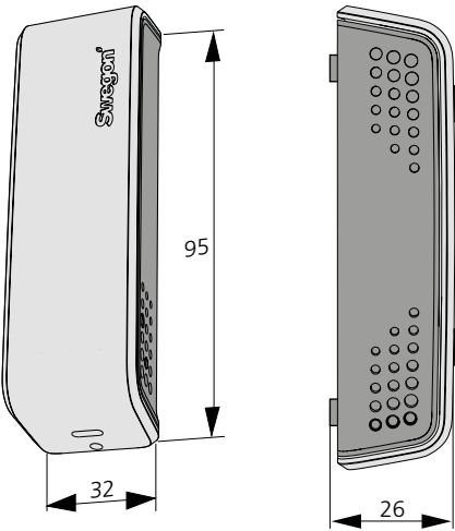
Figure 2. Dimensions, module principal WISE WCS
