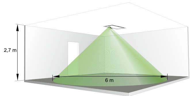
Figure 2. Detection range
