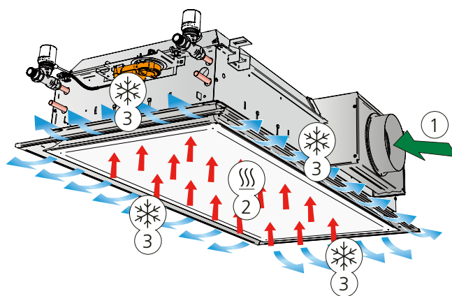
Figure 4. Variant A: Cooling and supply air function
