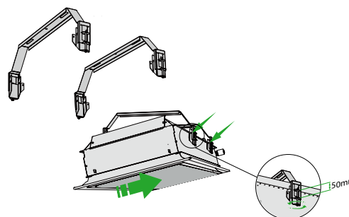
Figure 19. Installation with quick bracket PARASOL Z QUICK SUSPENSION KIT
