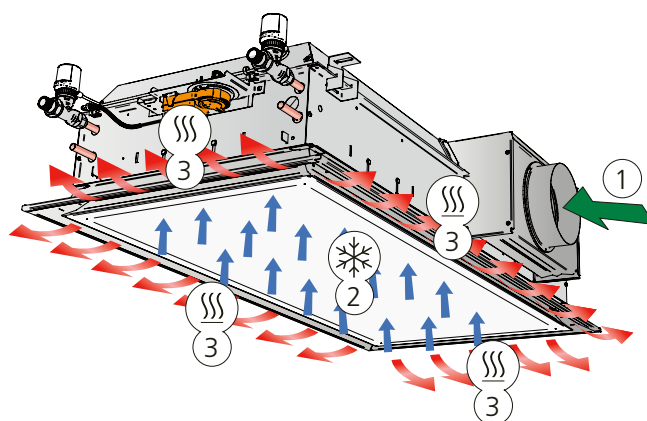
Figure 5. Variant B: Heating and supply air function (also including cooling function)
