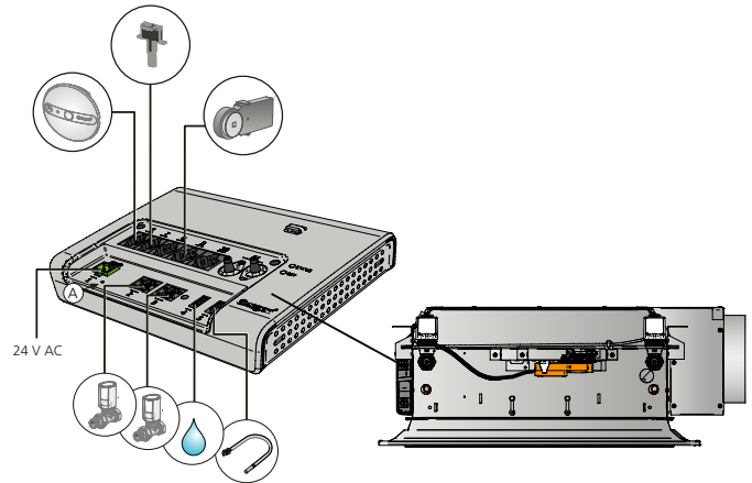
Figure 1. Components that are factory fitted on WISE Parasol Zenith A: Commissioning button
