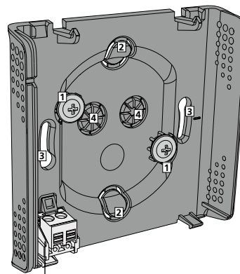
Figure 5. Back-piece. Connection of the power supply 24 V AC/15-30 V DC
