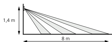
Figure 1. Detection range, wall mounted.
