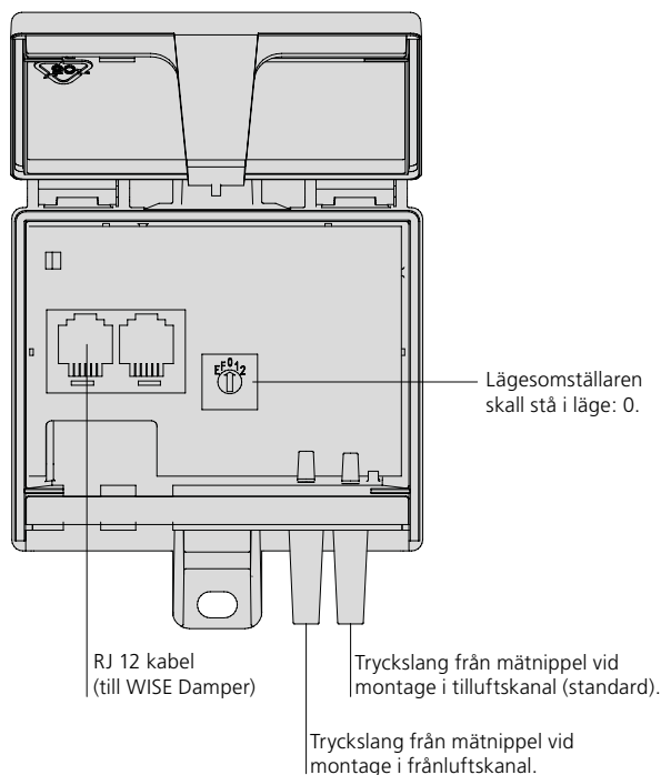
Figur 5. WISE DPS Modbus, inkoppling.
