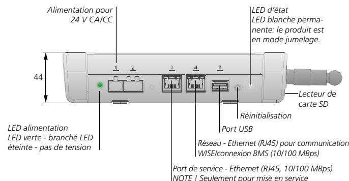
Figure 2. Raccordement des câbles et dimensions.
