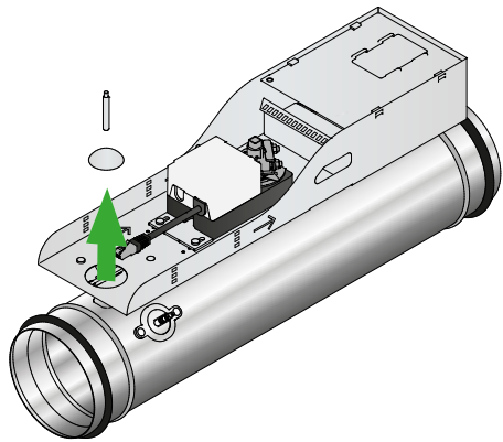
Figure 12. Dismantle the sealing plug from tubular damper casing.
