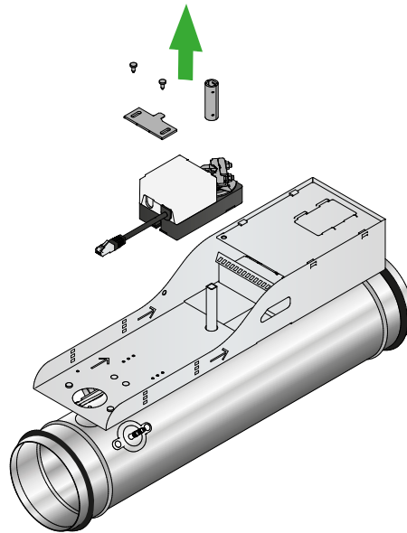
Figure 16. Dismantling the damper motor.
