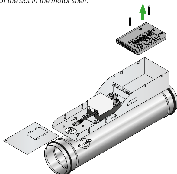
Figure 19. Remove tubes and contactors from WISE CU. Unscrew the 2 screws holding WISE CU in place (screw: PH1).
