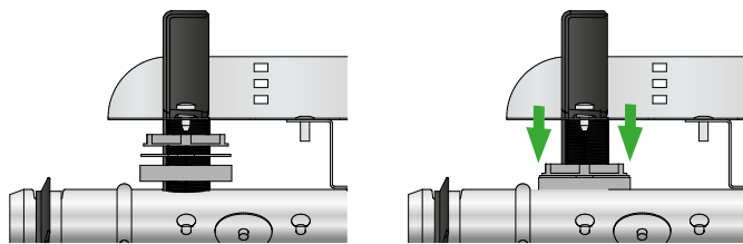
Figure 14. Tighten the counter nut against the tubular damper casing so that it presses the seal against the tubular damper casing.
