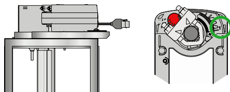
Figure 24. For damper position "Normally open" the damper should be open during installation of the spring return actuator. The spindle clamp then sits as shown above. NOTE! The spindle clamp needs to be moved to the rear of the motor, see figure 29-31.
