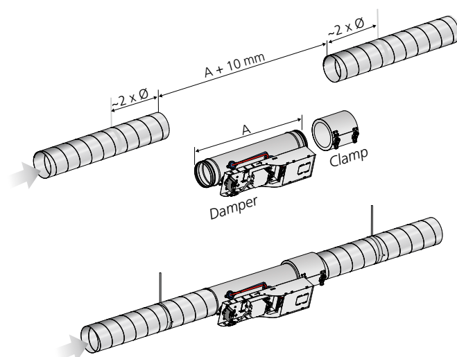
Figure 4. Installation in the duct system. The ducts must be firmly fixed to the frame of the building on each side of the product.
