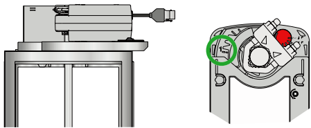
Figure 23. For damper position "Normally closed" the damper should be closed during installation of the spring return actuator. The spindle clamp then sits as shown above.
