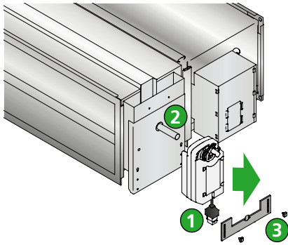
Figure 21. Dismantling the spring return actuator.
