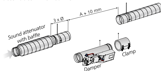
Figure 3. Straight duct section requirements 3 \times \varnothing in case of sound attenuator with baffle or centre body.
