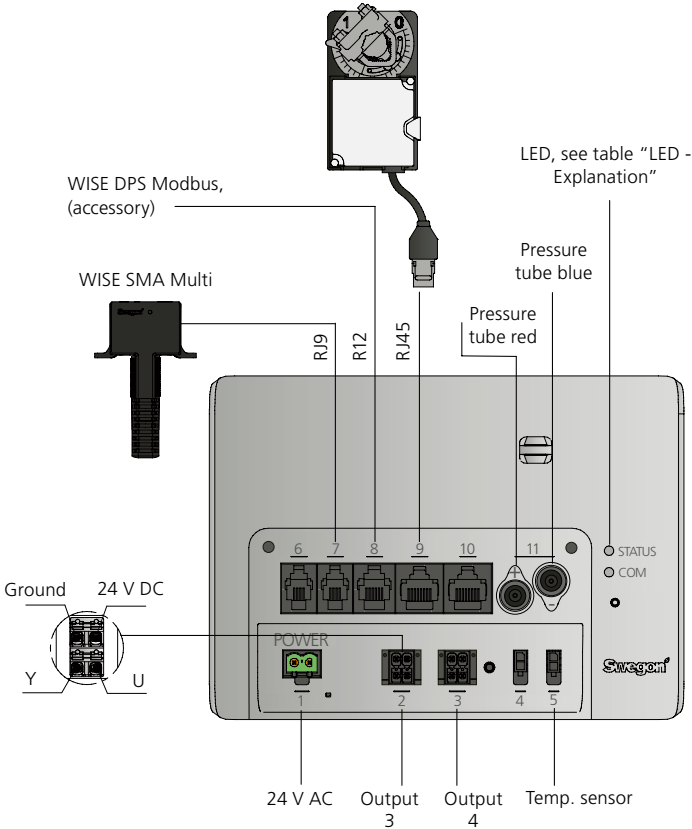
Figure 10. WISE Damper, connections.
