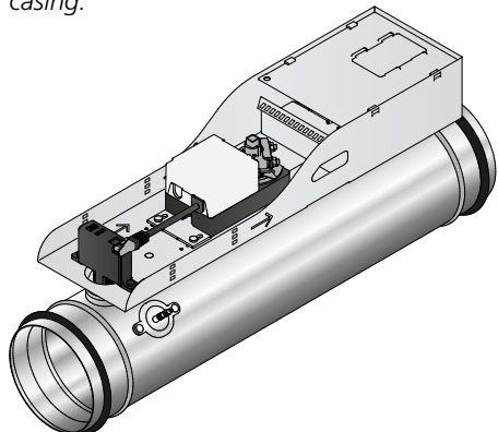
Figure 15. WISE SMA Multi installed. Electrical connection see "Connection".
