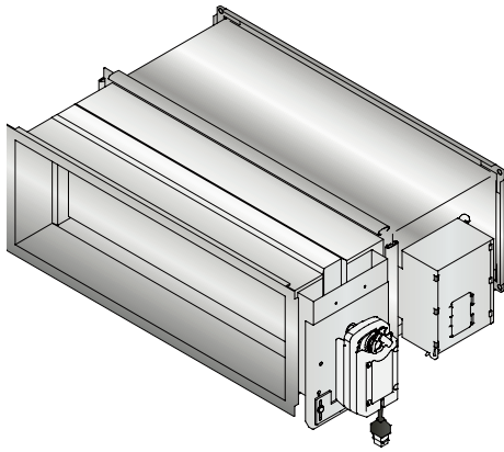
Figure 22. Install the new spring return actuator.
