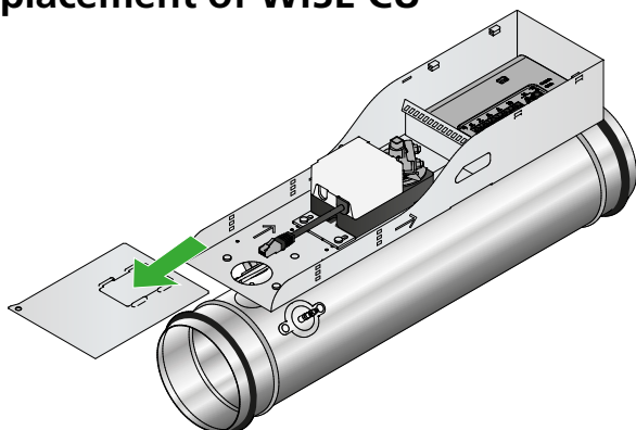
Figure 18. Dismantle the cover on the motor shelf by pulling it out of the slot in the motor shelf.
