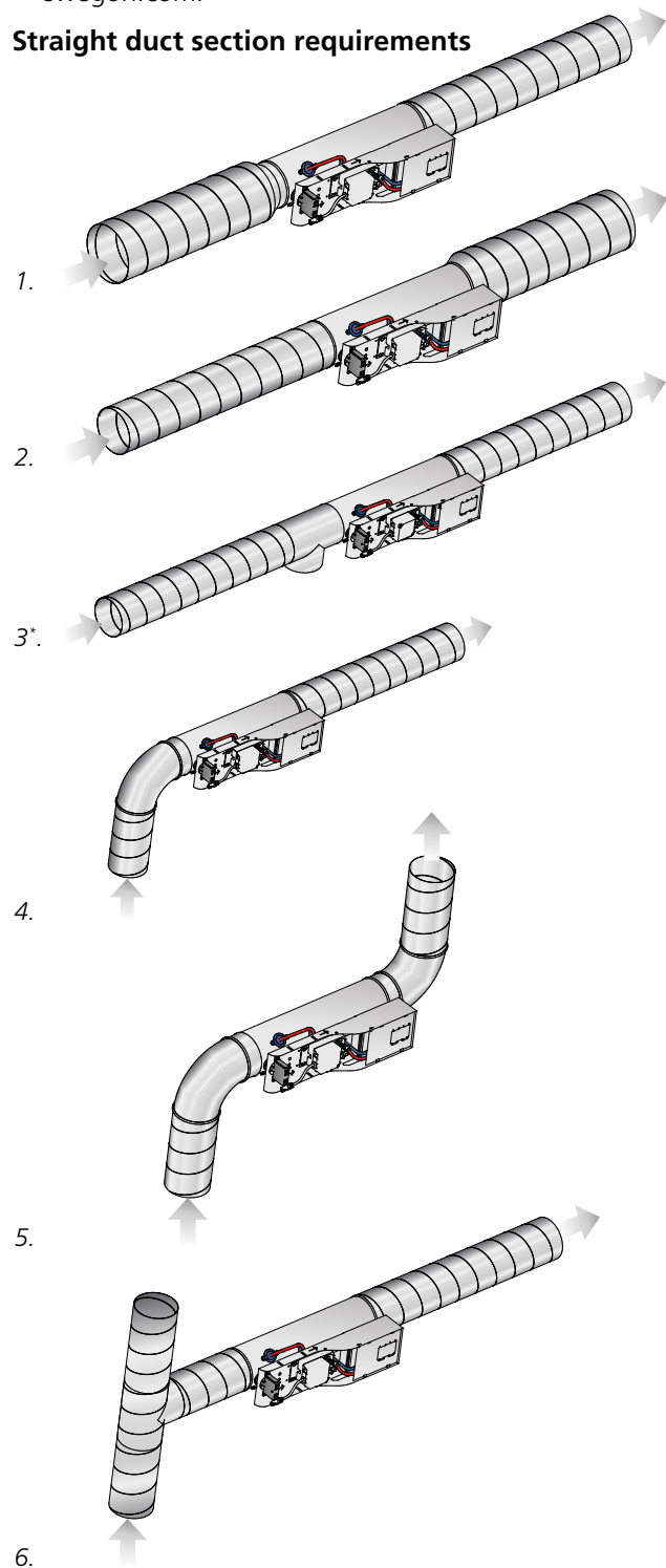
Figure 2. Straight duct section requirements in circular ducts, number of \varnothing before product: 1-5: Require no straight duct section. 6: Requires a straight duct section before the damper equivalent to 2 \times \varnothing . *T piece with a cleaning hatch.
