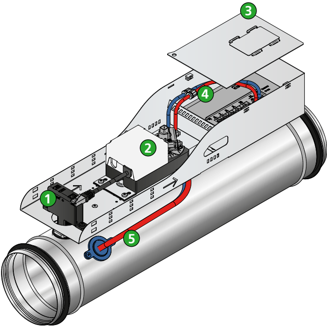
Figure 9. WISE Damper 1. WISE SMA Multi (alt. temperature sensor) 2. Damper motor 3. Cover 4. WISE CU 5. Measuring tubes
