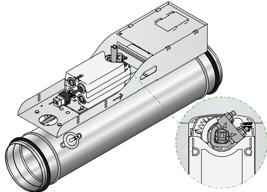
Figure 26. Install the new spring return actuator.
