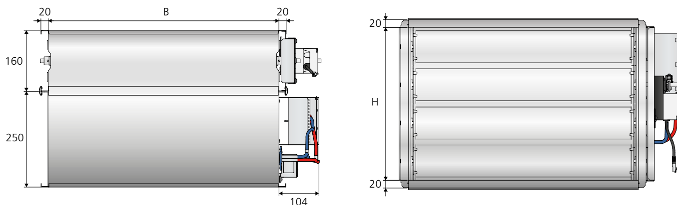
Figure 5. Dimensions, WISE Damper rectangular and WISE Damper rectangular with spring return.
