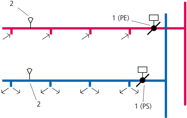
Figure 11. Constant pressure regulation. WISE Damper can be used to maintain a constant pressure, supplement with WISE DPS Modbus/WISE DPS. 1. WISE Damper. 2. WISE DPS Modbus/WISE DPS.
