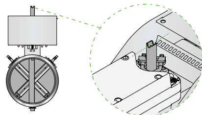
Figure 28. Damper blade position "Normally open".
