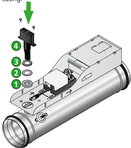
Figure 13. Install WISE SMA Multi in the following order:
