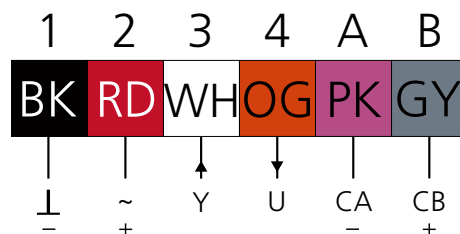
Figur 2. Inkoppling.
