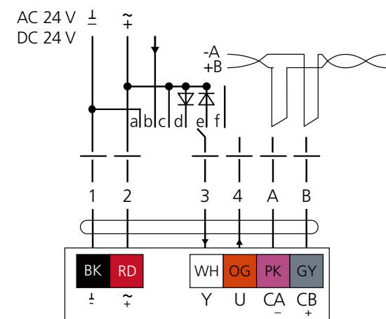
Figure 9. Wiring diagram.
