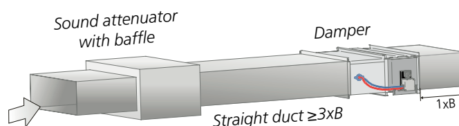
Figure 8. Straight duct section requirements 3 \times B in case of sound attenuator with baffle. Applies to both supply and extract air.
