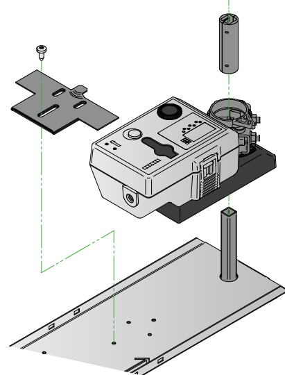
Figure 12. Dismantling the damper motor.
