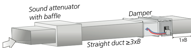
Figure 9. Straight duct section requirements 3 x B in case of sound attenuator with baffle. Applies to both supply and exhaust air.
