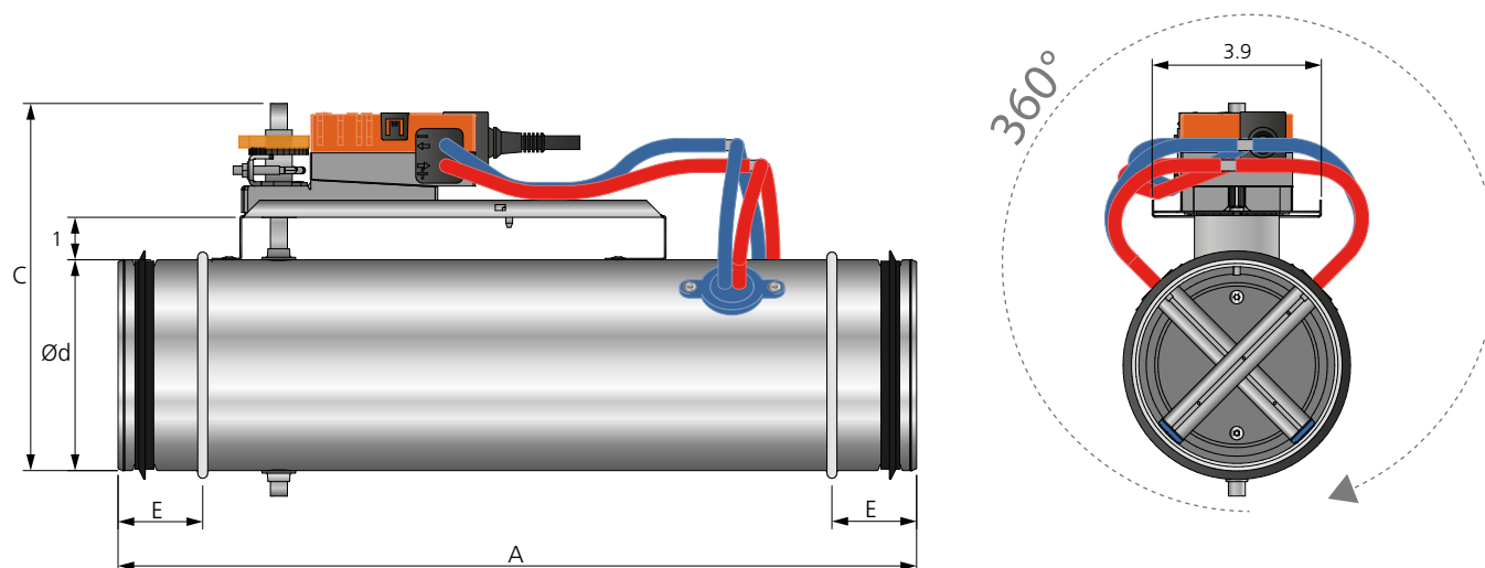
Figure 3. Dimensions (in), REACT V BMP circular. The damper can be installed at an optional angle.
