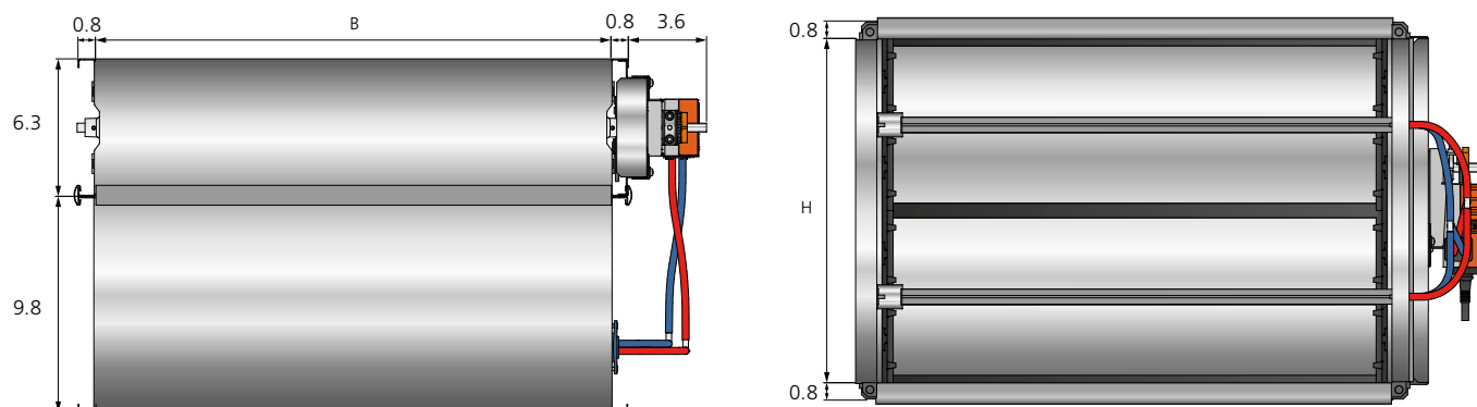
Figure 7. Dimensions (in), REACT V BMP rectangular.
