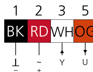
Figure 2. Connection.
