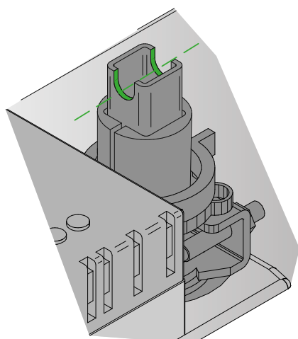
Figure 18. Recess in the damper shaft indicates the position of the damper.
