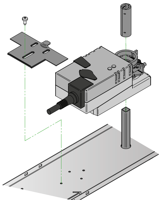
Figure 17. Dismantling the damper motor.
