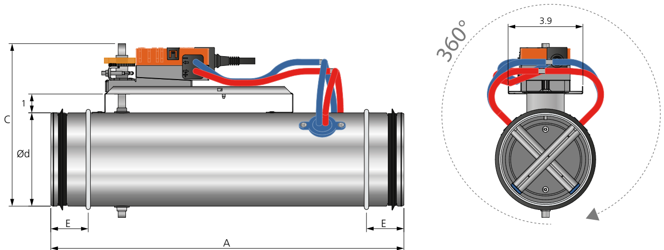
Figure 1. Dimensions (in), REACT V BMP circular. The damper can be installed at an optional angle.
