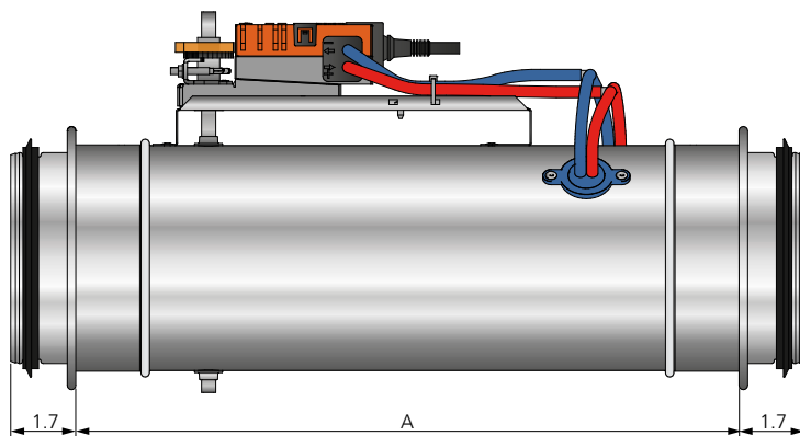
Figure 2. Dimensions with DUCT ADAPTER installed (in), REACT V BMP circular.
