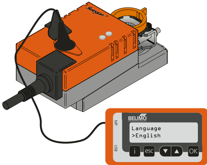
Figure 15. Belimo ZTH EU – Hand-held terminal for setting and reading the actuator's parameters.
