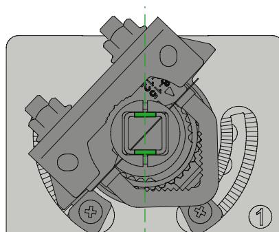
Figure 19. Damper open. Jumper to the left.
