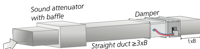
Figure 8. Straight duct section requirements 3 \times B in case of sound attenuator with baffle. Applies to both supply and exhaust air.
