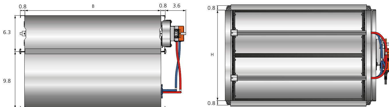
Figure 6. Dimensions (in), REACT V BMP rectangular.
