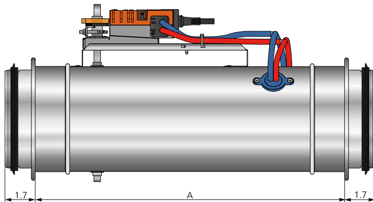
Figure 4. Dimensions with DUCT ADAPTER installed (in), REACT V BMB circular.
