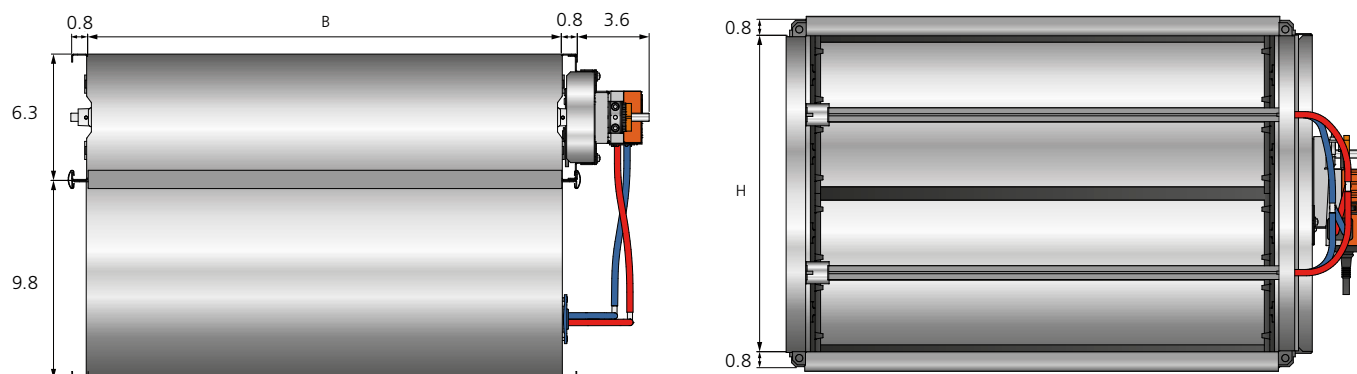
Figure 8. Dimensions (in), REACT V BMB rectangular.
