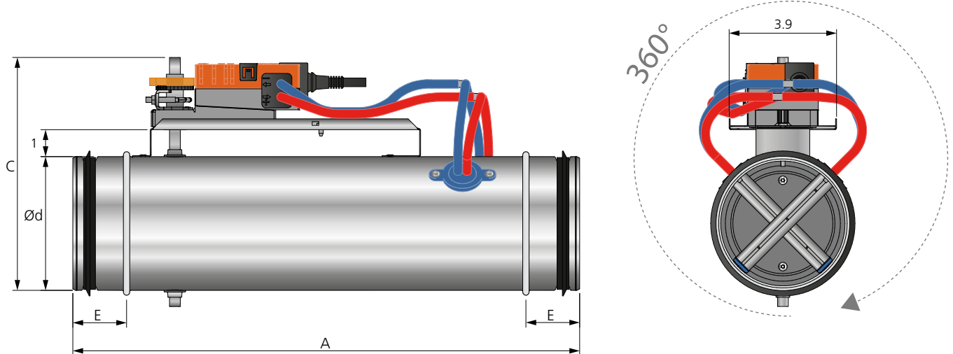
Figure 3. Dimensions (in), REACT V BMB circular. The damper can be installed at an optional angle.
