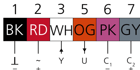
Figur 2. Tilkobling.
