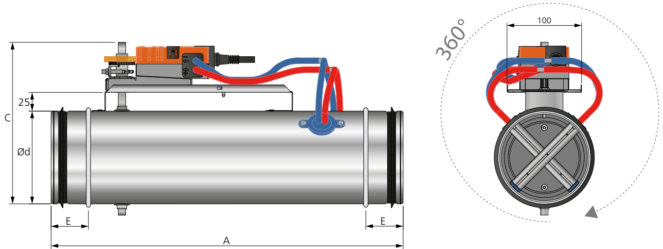
Figure 3. Dimensions (mm), REACT V BBAC circular. The damper can be installed at an optional angle.
