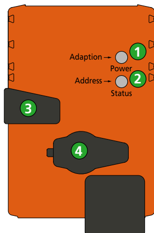
Figur 9. Belimo-aktuator.
