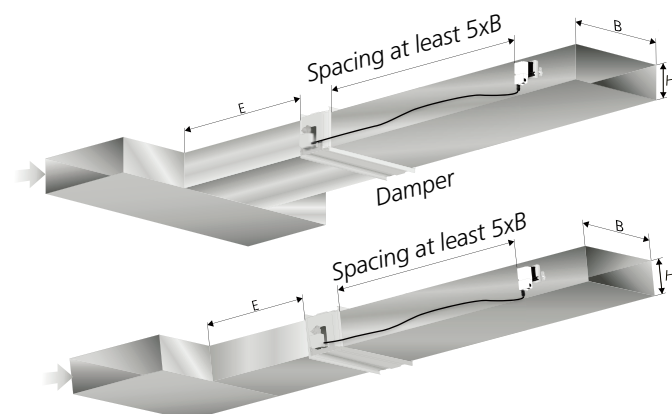
Figure 7. Straight duct section and distance requirements in rectangular ducts.
