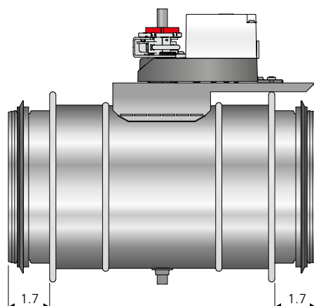
Figure 2. Dimensions (in), REACT PX GMB circular with DUCT ADAPTER installed.
