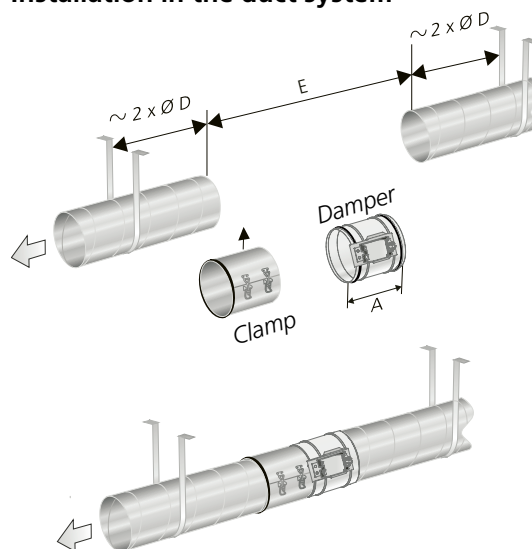
Figure 4. Installation in the duct system. The ducts must be firmly fixed to the frame of the building on each side of the product.
