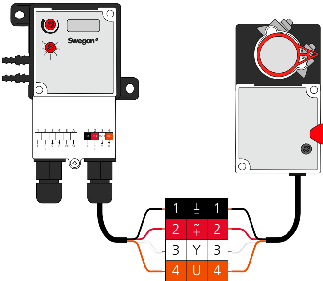
Figure 9. Connection between actuator and controller.
