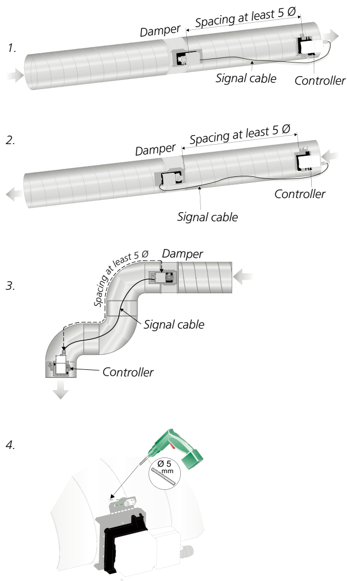
Figure 3. Distance requirements in circular ducts, number of Ø before and after product:
