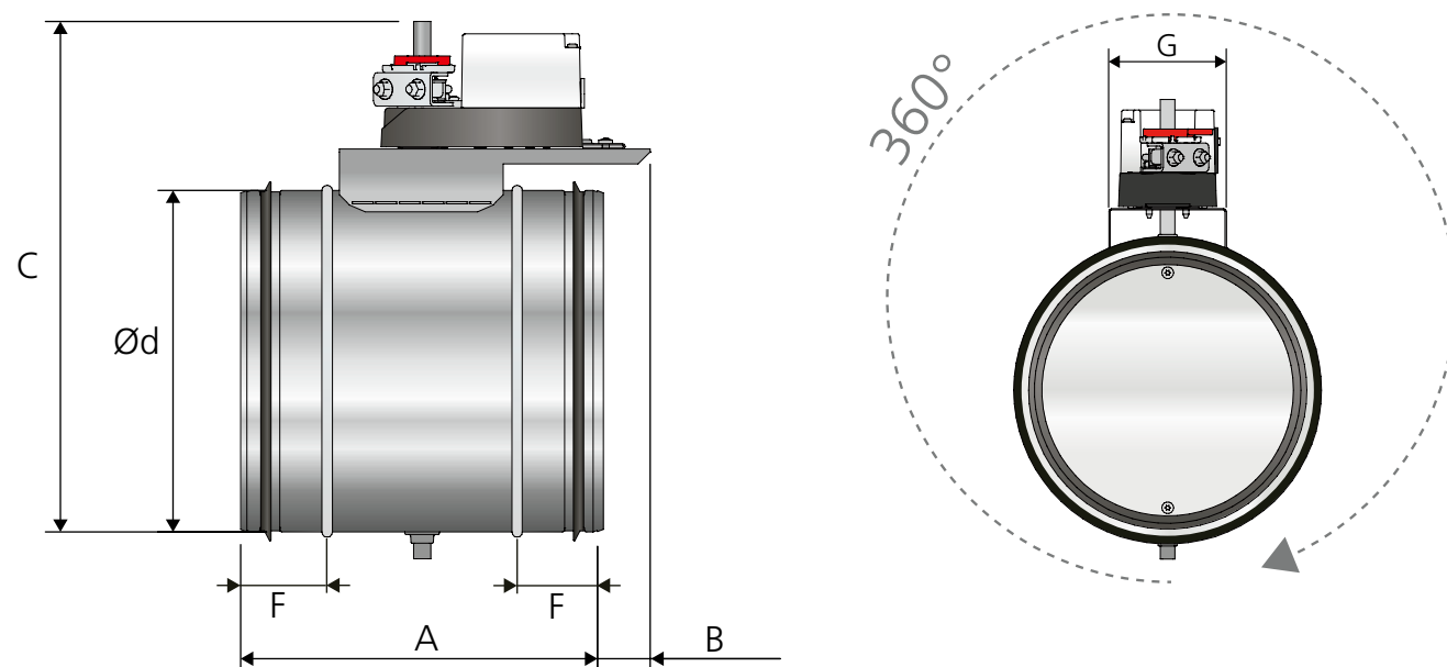
Figure 1. Dimensions (in), REACT PX GMB circular. The damper can be installed at an optional angle.
