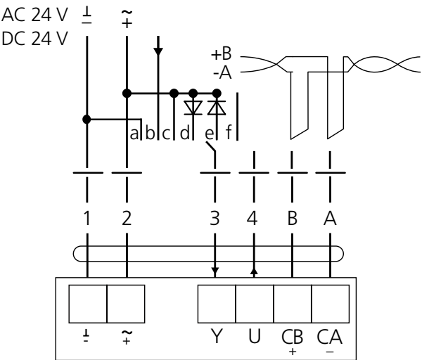
Figure 8. Connection.
