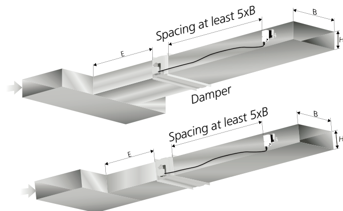
Figure 6. Straight duct section and distance requirements in rectangular ducts.
