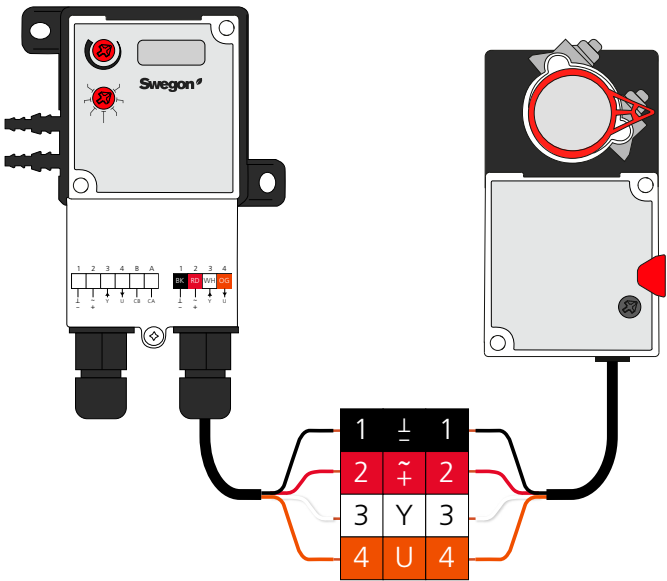
Figure 8. Connection between actuator and controller.
