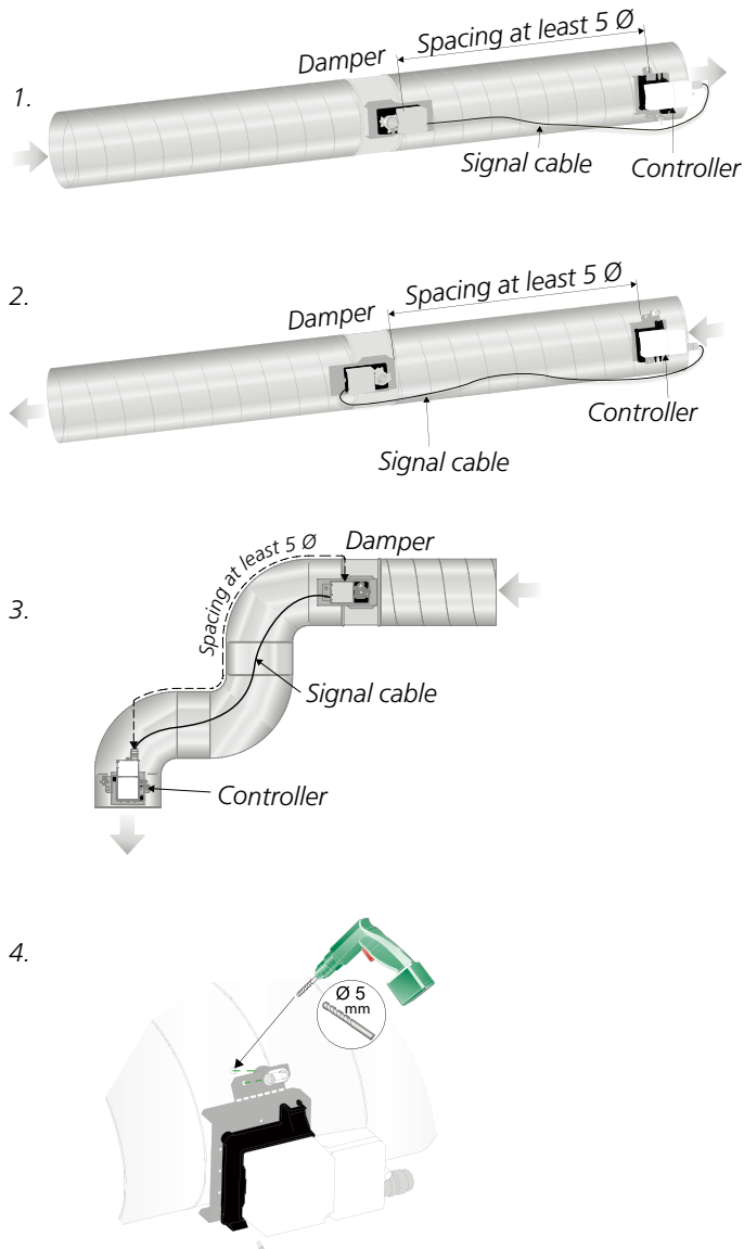
Figure 2. Distance requirements in circular ducts, number of \emptyset before and after product:
