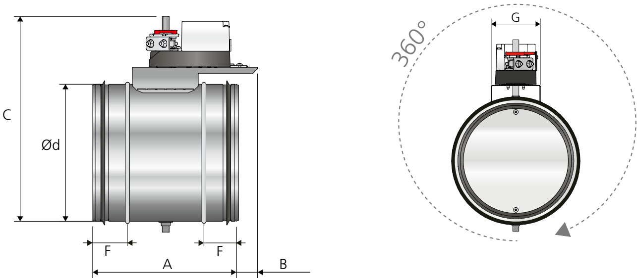
Figure 1. Dimensions (mm), REACT PX GMB circular. The damper can be installed at an optional angle.
