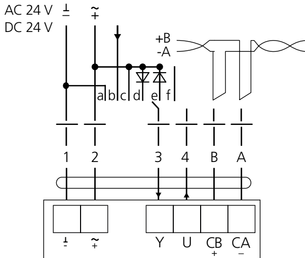
Figur 4. Inkoppling.
