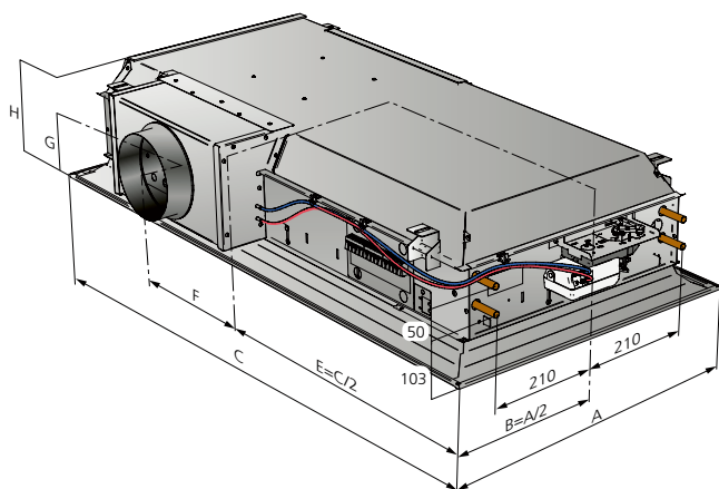
Figure 26. Dimensional drawing - long side connection (the length 1200 with air connection on side 4 is shown in the example).
