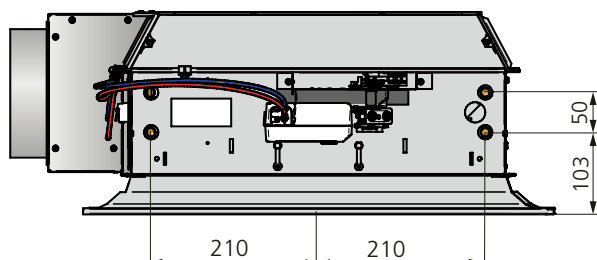
Figure 22. Dimensions, water connection length 600, 1200, 1800
