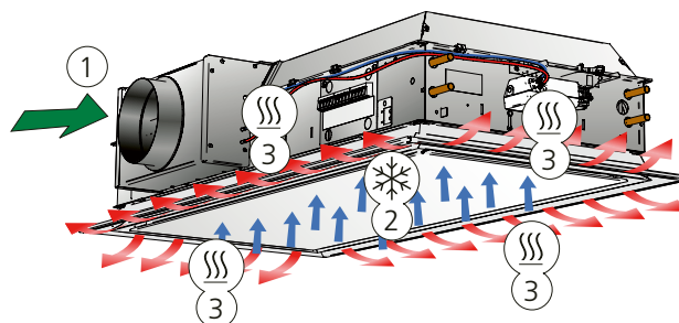
Figure 3. Variant B: Heating and supply air function
