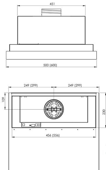
Samba Central CAVH silencer as standard
