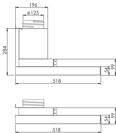
Samba (all models), side view
