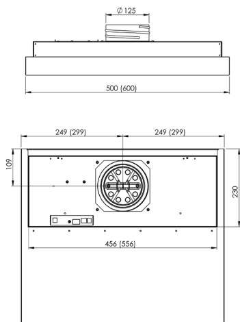
Samba Central CAVH silencer as standard
