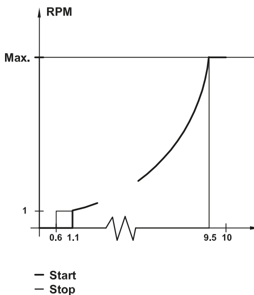
Fig. 1. Signal 0 - 10 V
